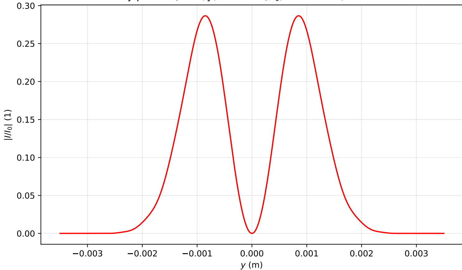
Intensity profile I(x=0, y, z=2.946)/I_0 , P_{in}=1.0P_{cr} , artificial time
